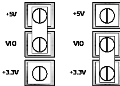
Figure 3.5: V I/O voltage selection
